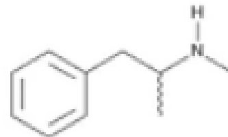
methamphetamine
