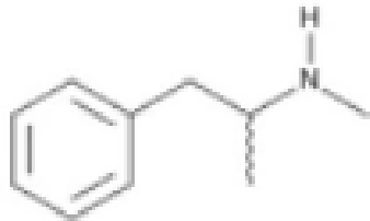
methamphetamine
