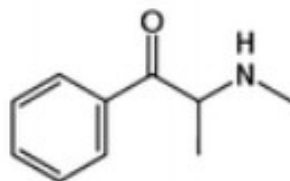
methcathinone
