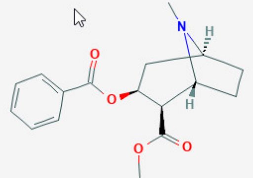
Cocaine
