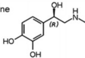
epinephrine
