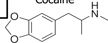
MDMA (Ectasy)
