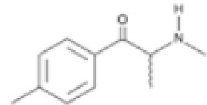
mephedrone
