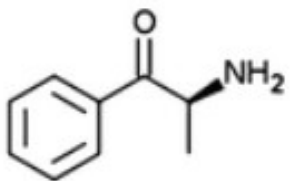
cathinone
