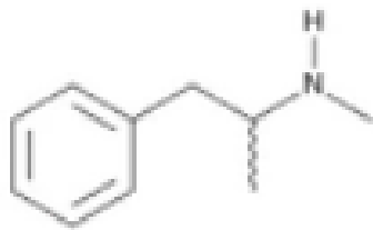
methamphetamine
