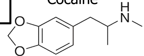
MDMA (Ectasy)
