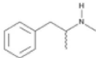
methamphetamine
