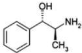
cathine
