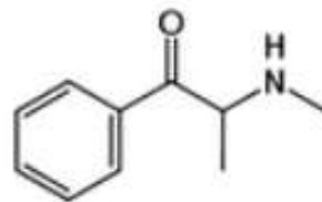
methcathinone
