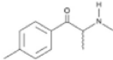
mephedrone
