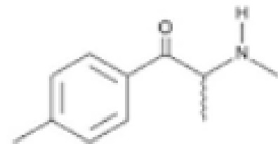
mephedrone
