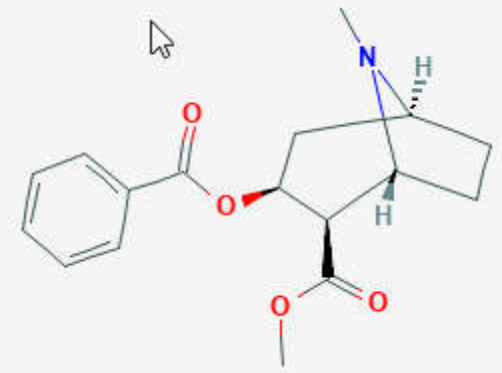
Cocaine
