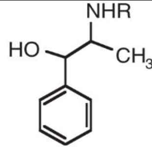
Pseudoephedrine or Ephedrine: R=CH 3
